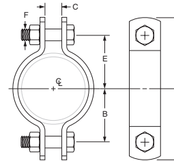
FIG. 212: LOADS (LBS) • WEIGHT (LBS) • DIMENSIONS (IN)
