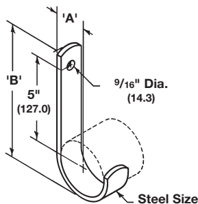
Figure B3191 Straight J-Hook
