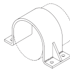
Figure B3256 Hold-Down Anchor Clamp Page 108
