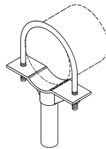
Figure B3090 Pipe Saddle Support With U-Bolt Page 96-97
