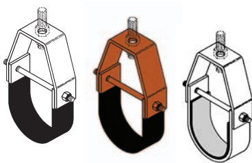
Figure B3104C Plastic Coated Light Duty Clevis Hanger Page 42
