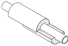
Figure B3380 thru B3384 360° Calcium Silicate Shield Page 91
