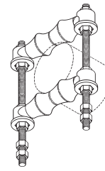
Figure B3122A Adjustable Double Roller Guide Page 76
