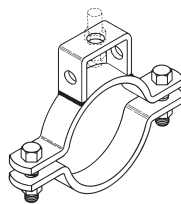
Figure B386 Suspension Rod Pipe Clamp Page 55
