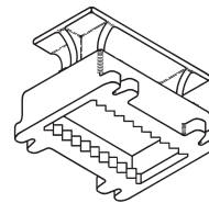
Figure B3014 Malleable Iron Spot Insert Page 131
