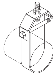
Figure B3108 Extended Clevis Hanger Page 45
