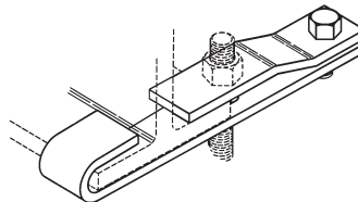
Figure B3045 Side Beam Clamp Page 35
