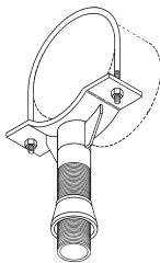
Figure B3092 Adjustable Pipe Saddle Support With Yoke Page 100-101
