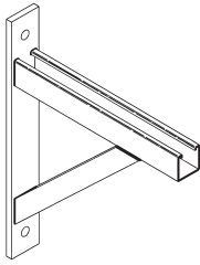
Figure B3064 Adjustable Strut Bracket Page 139
