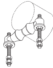
Figure B3122 Adjustable Roller Support Page 75
