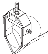
Figure B3106 Vee Bottom Clevis Hanger Page 47
