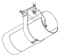
Figure B3153 Insulation Protection Shield With Tabs Page 125
