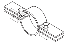
Figure B3132 Two-Bolt Underground Clamp Page 63
