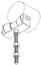
Figure B3124 Roller Support Page 78
