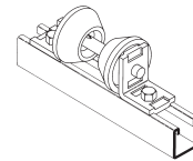
Figure B219 Pipe Rollers Page 81
