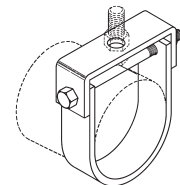
Figure B3109 Flat Top Clevis Hanger Page 46
