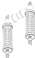
Figure B3264 Spring Cushion Hanger Page 87
