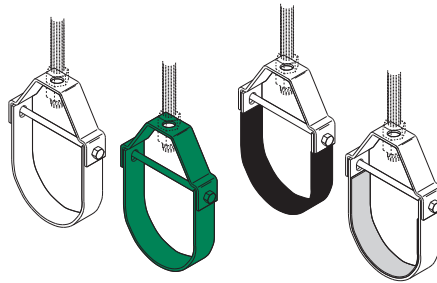
Figure B3100 Standard Clevis Hanger Page 40 & 41 *
