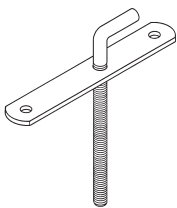
Figure B3019 Adjustable Metal Deck Ceiling Bolt Page 129
