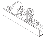
Figure B218 Pipe Rollers Page 80
