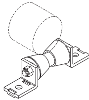
Figure B3126 Roller Support Page 79
