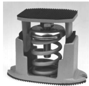
Figure HMLT/HMT Housed 1" Deflection Mounting Pages 178 & 179
