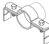
Figure B3149 Marine Hanger Page 69
