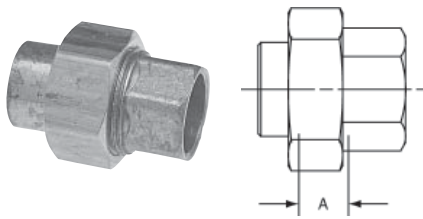
633-W Union C x C – Wrot
