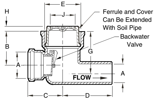
Fig. 7022S . . . HUB INLET - SPIGOT OUTLET
