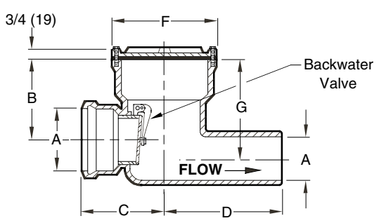
Fig. 7012S . . . HUB INLET - SPIGOT OUTLET
