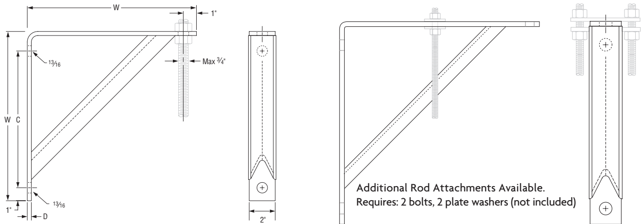
FIG. 194: LOAD (LBS) • WEIGHT (LBS) • DIMENSIONS (IN)
